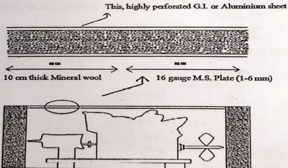
Fig. 4 Schematic Diagram of the DG set in an Acoustic Enclosure
