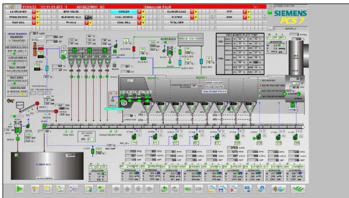
Fig 3.3: CCR Snapshot of Cooler
